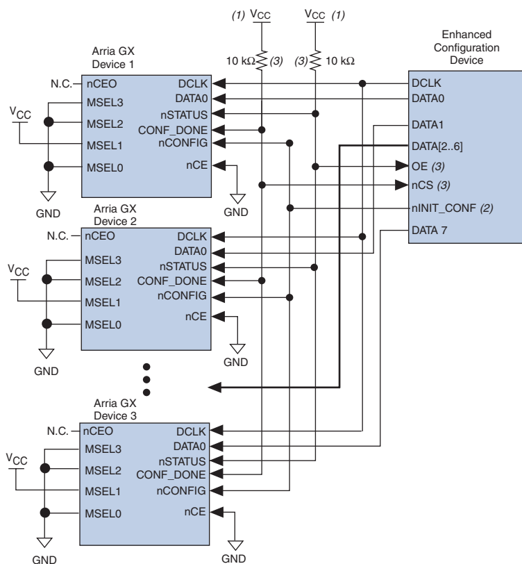
Figure 11–23. Concurrent PS Configuration of Multiple Devices Using an Enhanced Configuration Device
