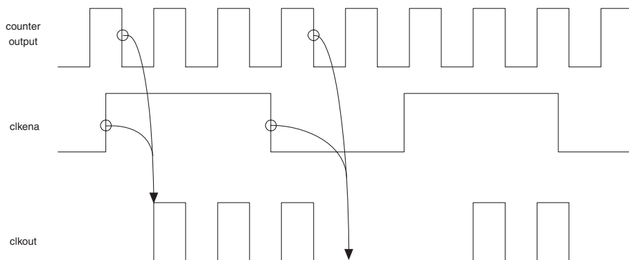
Figure 5–53. clkena Signals
