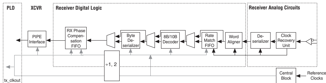
Figure 1–14. Individual Channel Receiver Logic Clocking with Rate Matching
