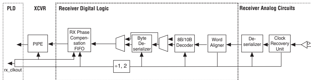
Figure 1–15. Individual Channel Receiver Logic Clocking Without Rate Matching
