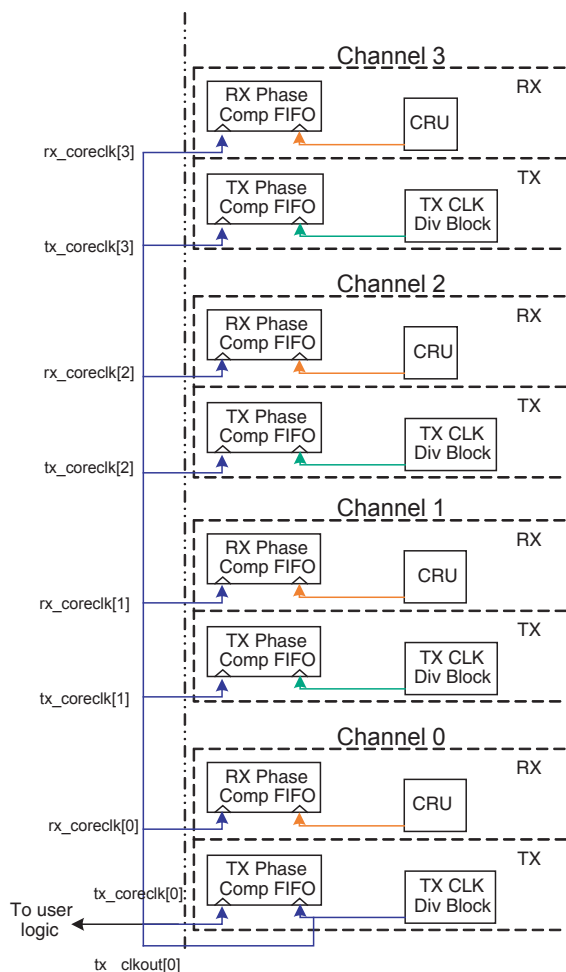
Figure 1–57. User Controlled Phase Compensation FIFO Clock
