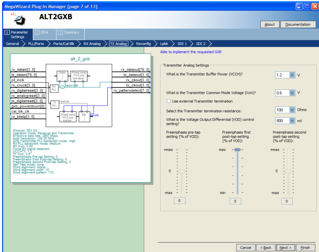
Figure 3–34. MegaWizard Plug-In Manager - ALT2GXB (TX Analog)
