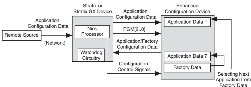
Figure 12–12. Remote System Configuration Using Enhanced Configuration Devices
