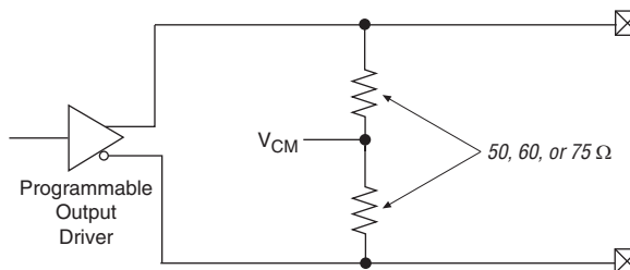
Figure 11. Programmable Transmitter Termination
