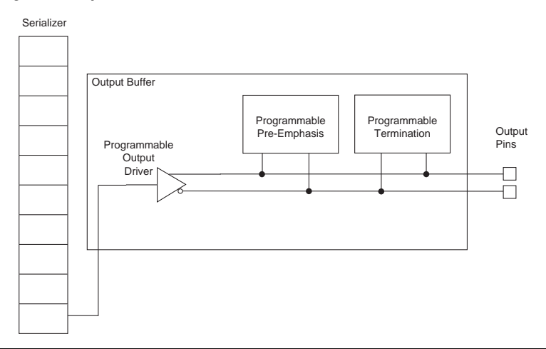
Figure 8. Output Buffer
